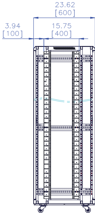
B-B (Right Section View)
