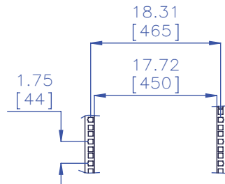
Rack Dimensions
