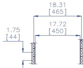
Rack Dimensions
