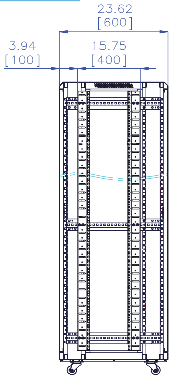
B-B (Right Section View)
