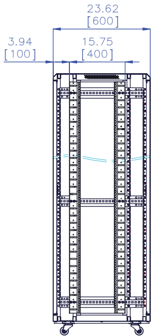
B-B (Right Section View)
