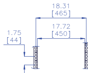
Rack Dimensions
