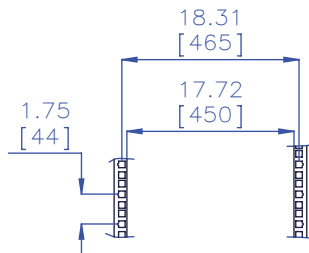
Rack Dimensions
